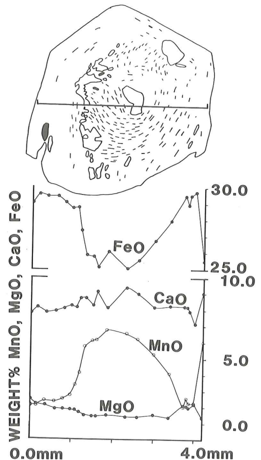
Fig. 11. Typical compositional profile of a texturally zoned garnet from garnet-amphibole micaschist, Nordåsvatn Complex. On the left hand side a textural and chemical break is clear and coinciding. On the right hand side the break appears somewhat less well defined. Near locality 1.
