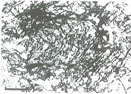
Fig. 10. Garnet from micaschist of the Nordåsvatn Complex, MiBA, showing an inner core with fine-grained inclusions defining a curved foliation, and an outer rim with more randomly oriented, coarser inclusions. Locality 4. Scale bar: 1 mm.
