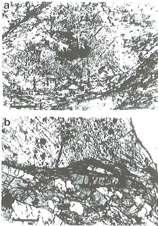
Fig. 6. (a) Amphibole porphyroclast recrystallizing to smaller amphiboles along the margins. A chemical variation between the porphyroclast and the newer grains along the margins is shown in Fig. 7. Protomylonitic gabbro, Nordåsvatn Complex, MiBA. Similar porphyroblasts occur in ophiolitic rocks in the MaBA. Locality 4. Scale bar: 1 mm. (b) Close-up of the edge of a large, relict amphibole porphyroclast in strongly deformed gabbro-pegmatite, Nordåsvatn Complex. A preferred orientation of the new-formed amphiboles indicates stress-related (syn-tectonic) growth. For chemical compositions, see Fig. 7. Locality 5. Scale bar: 1 mm.
