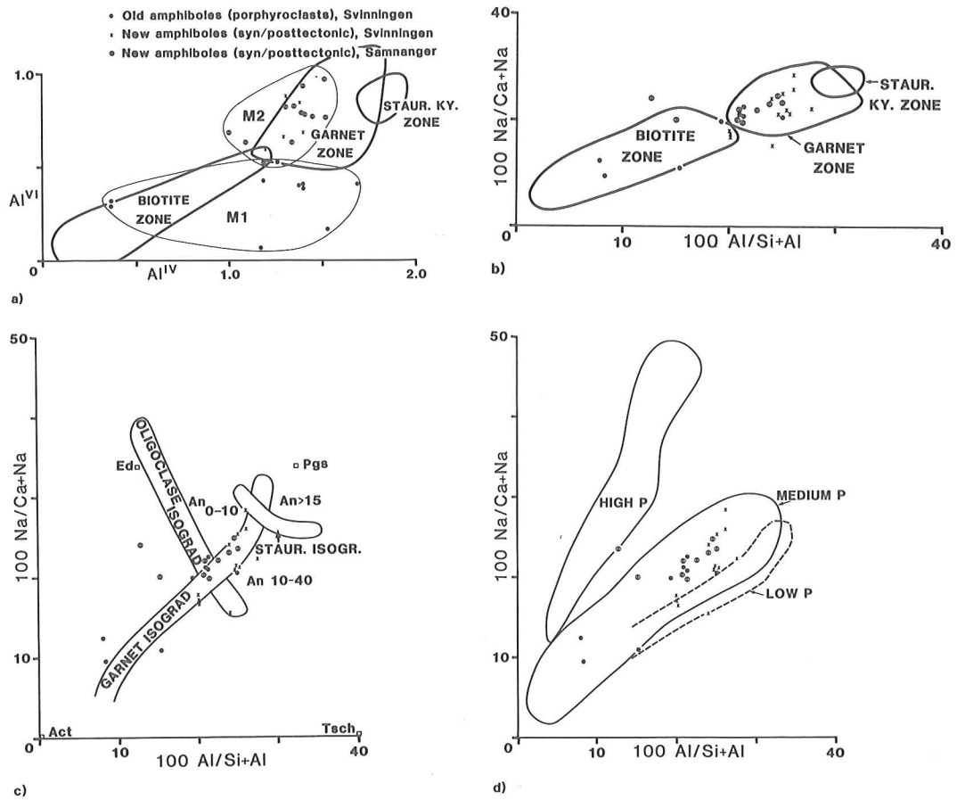
Fig. 8. Same as Fig. 7 but from the Gulffjellet Ophiolite Complex, MaBA. Localities 6 and 7.
